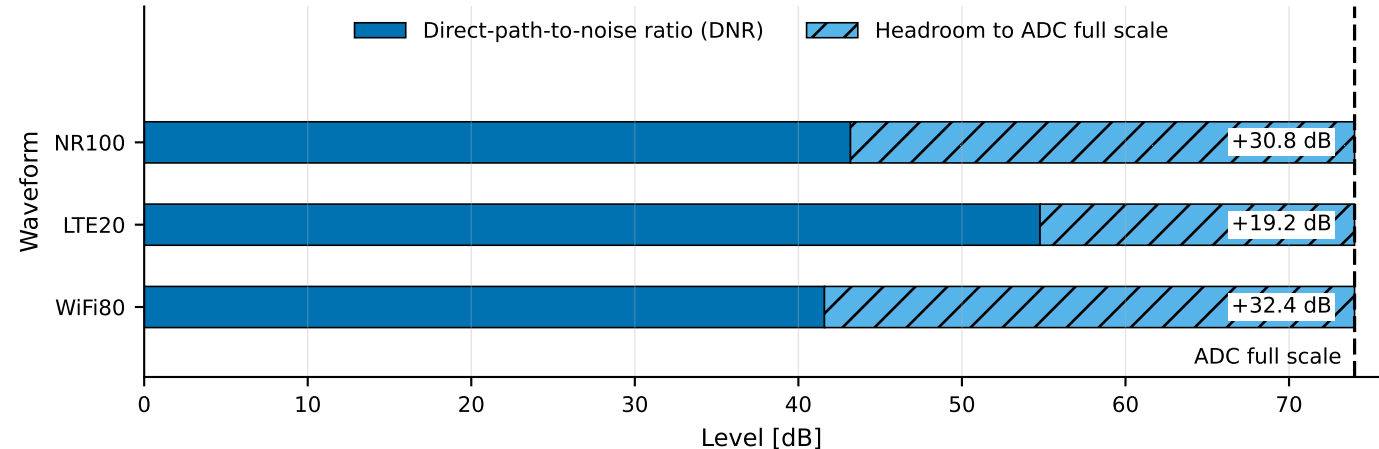
Headroom of the 12-bit ADC dynamic range (74.0 dB) above the direct-path-to-noise ratio
