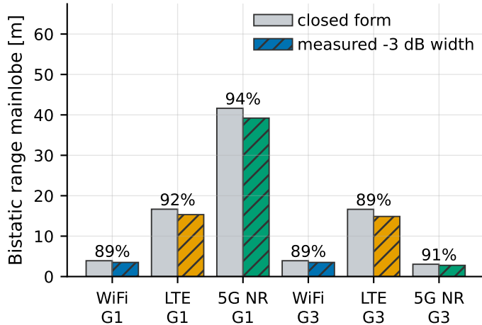
(a) Range: measured -3 dB width vs c/B_{\text{ref}}
