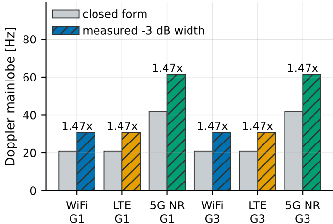
(b) Doppler: measured -3 dB width vs 1/T_{\text{CPI}}
