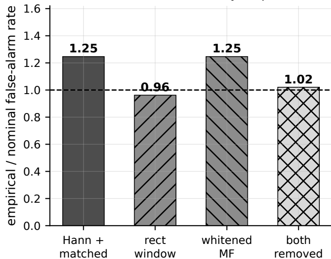
(a) 5G NR, noise-only maps
