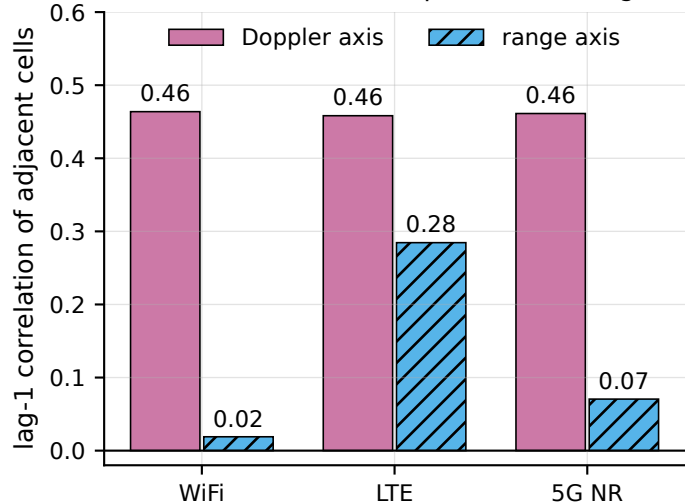
(b) CA-CFAR assumes independent training cells
