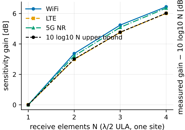
(a) Measured gain against the idealised coherent bound
