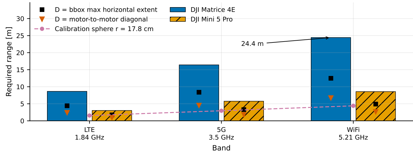
Far-field distance 2D^2/\lambda , D = envelope diagonal incl. rotor discs
