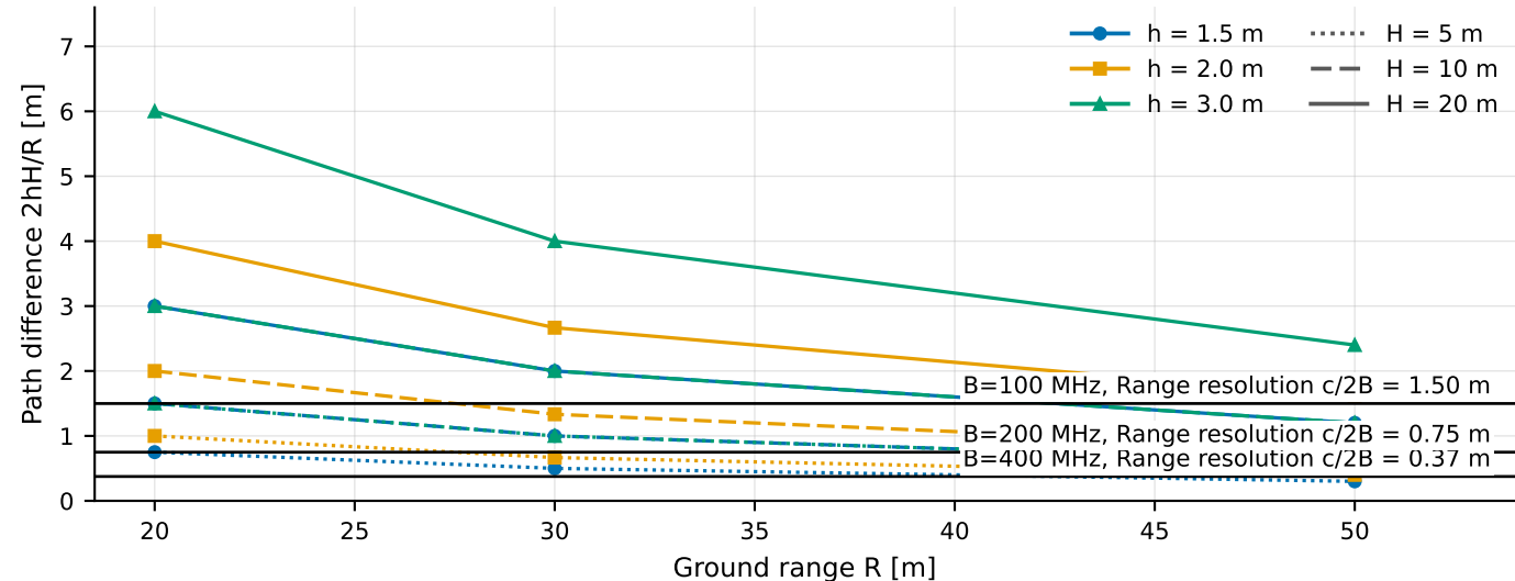
Target-via-ground ghost: path difference against range resolution Colour and marker give the antenna height h , line style the target height H
