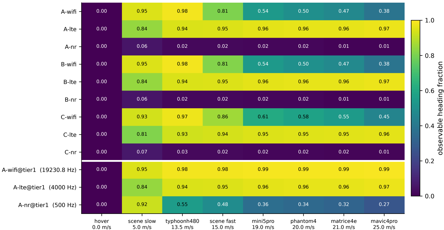
Fraction of headings that are BOTH unambiguous and detectable (CPI 0.1 s)
