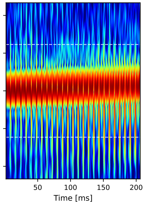
Ours (SBR+PO, default) 7.9 dB p-p · level +0 dB vs strongest
