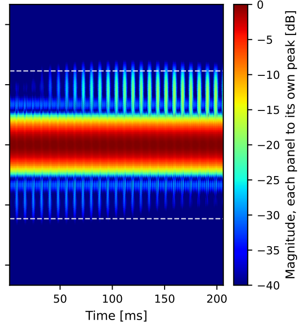
Ours w/o occlusion (control) 2.8 dB p-p · level -2 dB vs strongest
