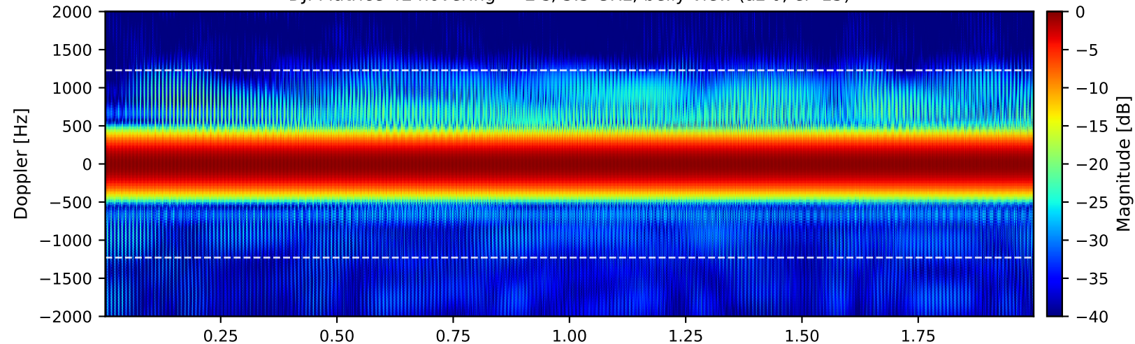
Rotor speeds — spread taken from measured PX4 telemetry (0.07-0.29 %)
