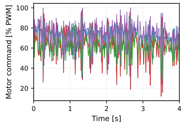
DJI Phantom 3 — outdoor, motor PWM command (not rpm)
