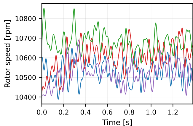
NeuroBEM racing quad — indoor, measured rpm
