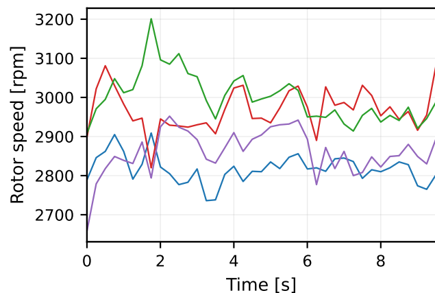
PX4 CODEV AQUILA V3 — outdoor, measured rpm
