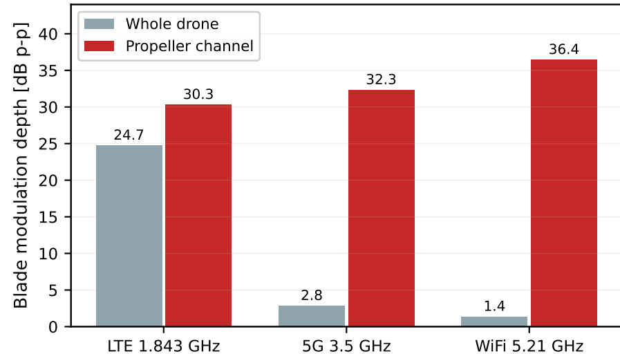
(a) The blade signal is strong. The body hides it.
