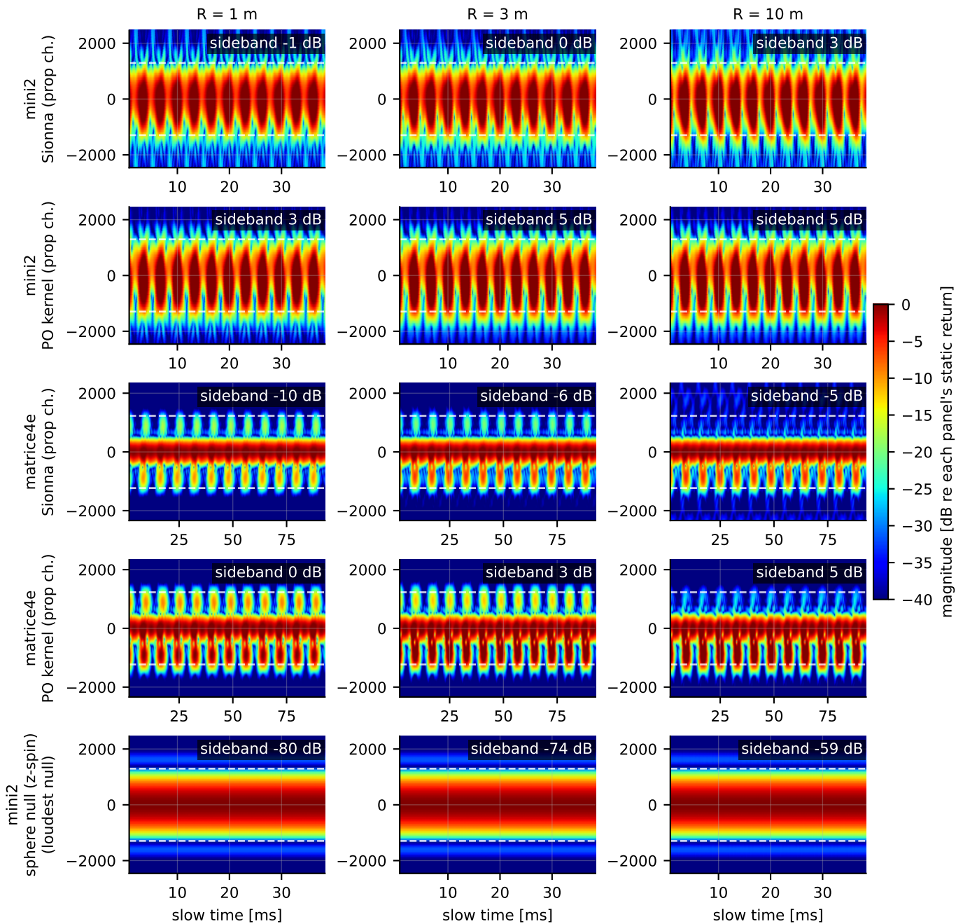
Two-sided micro-Doppler, aspect az 0 / el 15. White dashed = kinematic tip Doppler.
