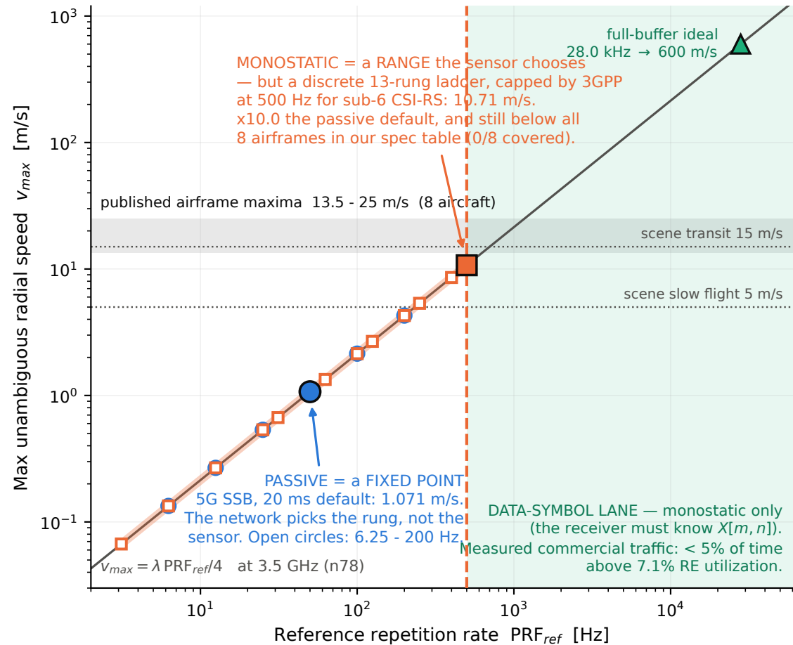
(a) The boundary at one carrier (n78, 3.5 GHz): who chooses \text{PRF}_{ref}
