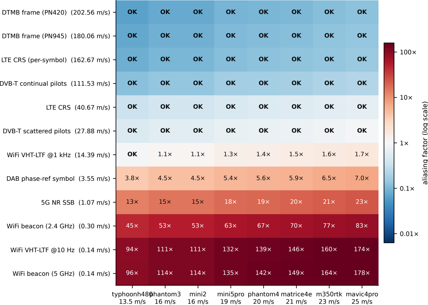
Aliasing factor v_{max, \text{airframe}} / v_{max, \text{illuminator}} bold OK = the airframe's published maximum is measurable unambiguously
