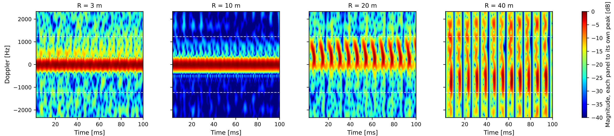
DJI Matrice 4E hovering — Sionna PathSolver range sweep, true monostatic (TX = RX, baseline 0), belly view (az 0, el -15), 3.5 GHz
