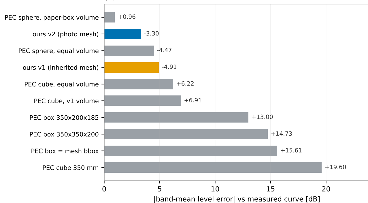
(d) Does the mesh still beat a metal box?
