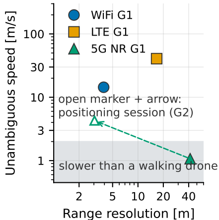
(c) The 5G double penalty
