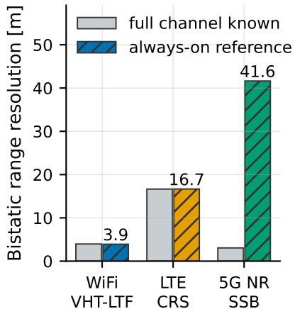
(b) 5G is 2.5x coarser
