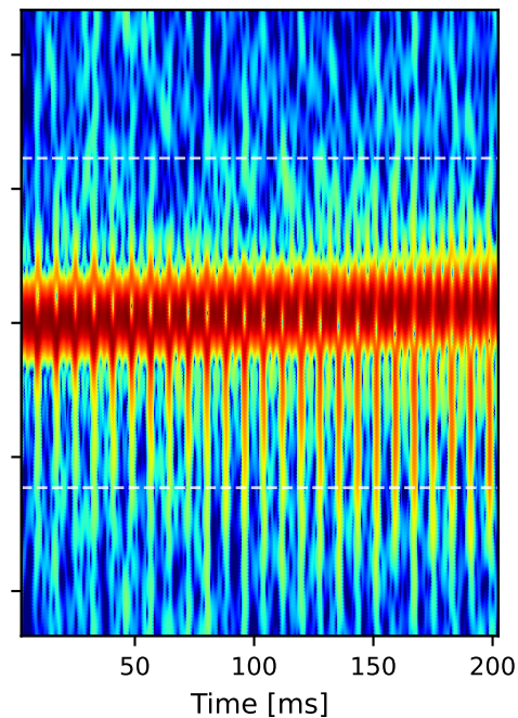
Ours (SBR+PO, default) 8.0 dB p-p · level +0 dB vs strongest
