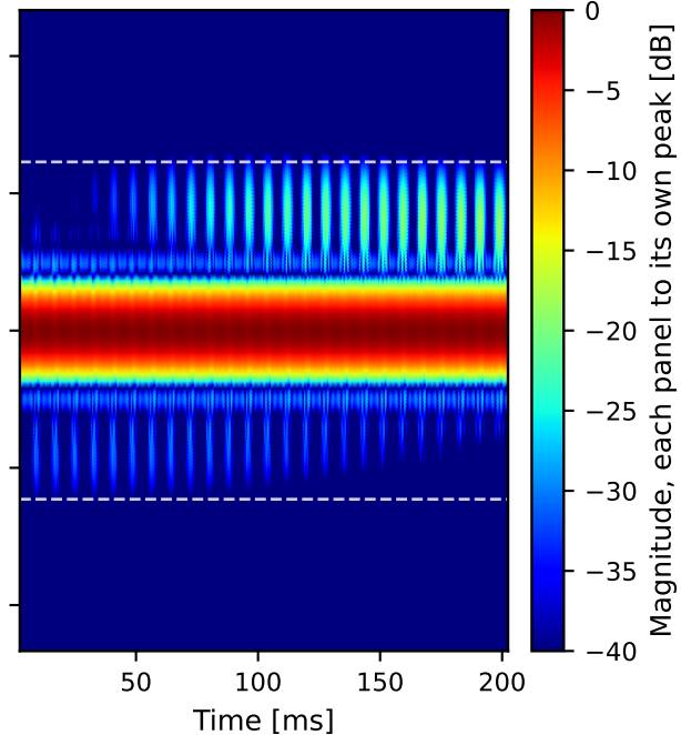
Ours w/o occlusion (control) 2.7 dB p-p · level -2 dB vs strongest
