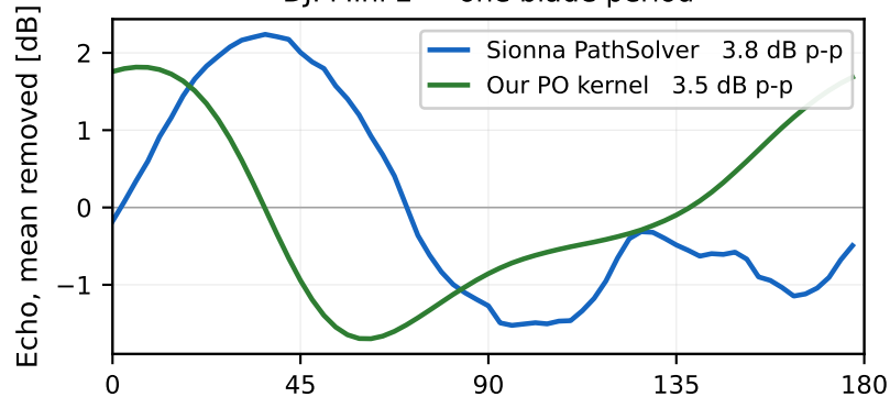
Rotor stepped and re-traced by two independent engines — 3.5 GHz, range 3 m, nose aspect DJI Mini 2 — one blade period
