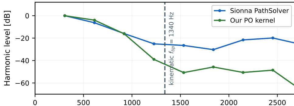
Rotor stepped and re-traced by two independent engines — 3.5 GHz, range 3 m, nose aspect DJI Mini 2 — one blade period
