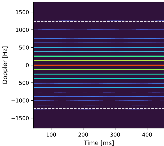
All four rotors at one rpm half-window spectrum correlation 0.9966
