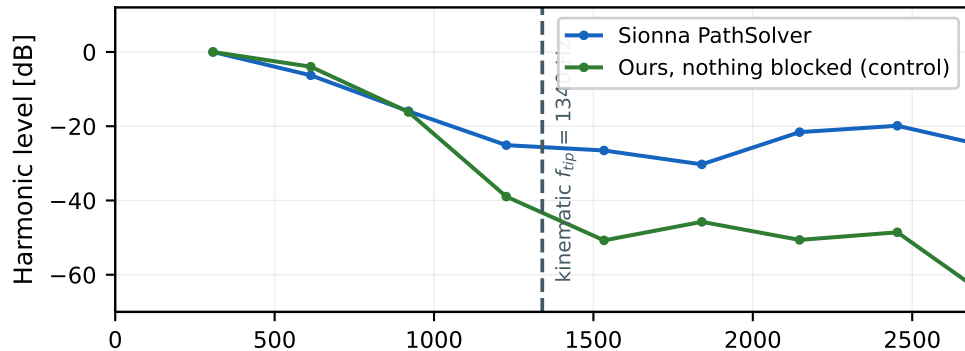
Stock path solver vs our unoccluded PO control (no SBR arm) — 3.5 GHz, range 3 m, nose aspect, 0.2 m baseline DJI Mini 2 — one blade period
