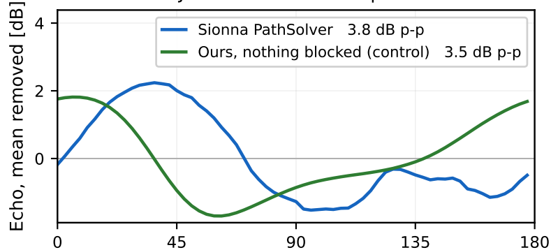
Stock path solver vs our unoccluded PO control (no SBR arm) — 3.5 GHz, range 3 m, nose aspect, 0.2 m baseline DJI Mini 2 — one blade period
