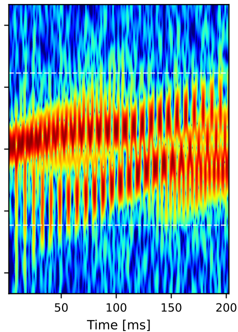
Ours (SBR+PO, default) 7.5 dB p-p · level +0 dB vs strongest
