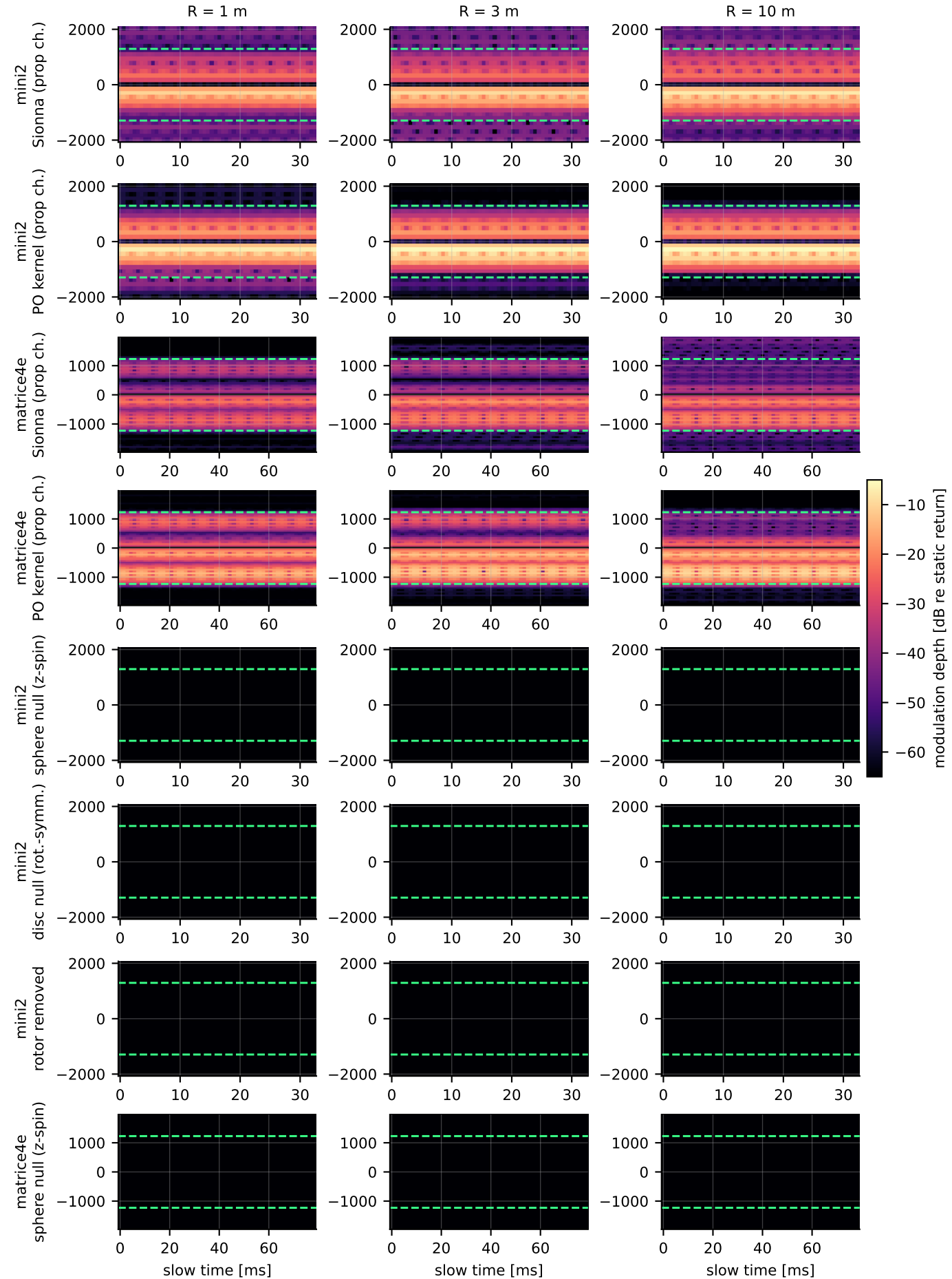
Two-sided micro-Doppler spectrograms, aspect az=0 el=15 Shared colour scale, in dB relative to each panel's own static (DC) return, so null rows compare directly with signal rows. Green dashed = kinematic tip Doppler.
