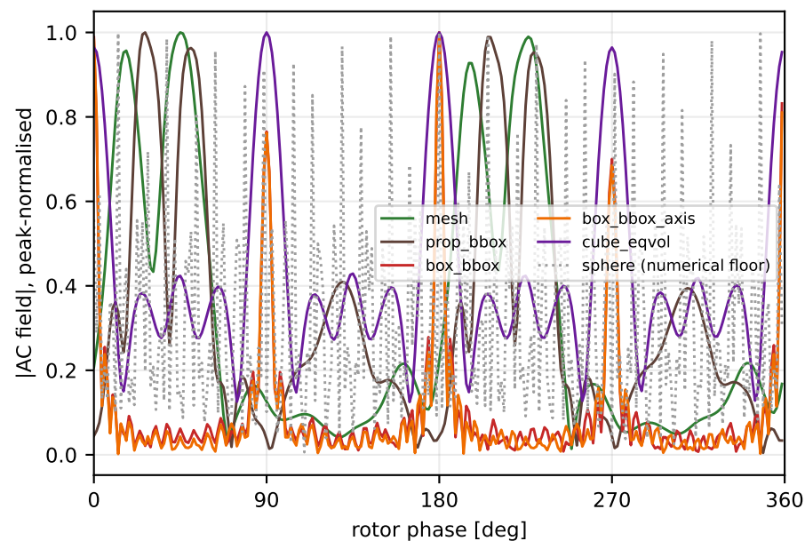
(a) one revolution, az = 0^\circ
