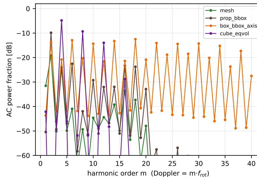
(b) line spectrum — 90^\circ vs 180^\circ symmetry
