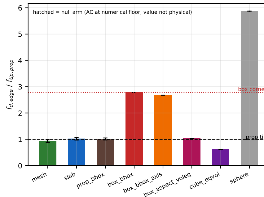
(e) Doppler width vs prop-tip prediction
