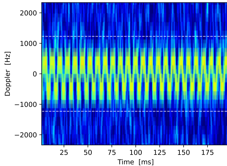
(h) Target only, ECA off — control for the zero-Doppler notch
