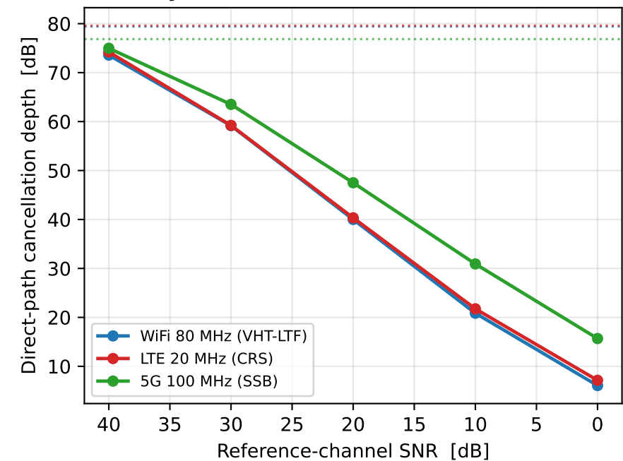
(c) Why it costs: ECA cannot cancel what it mismeasures
