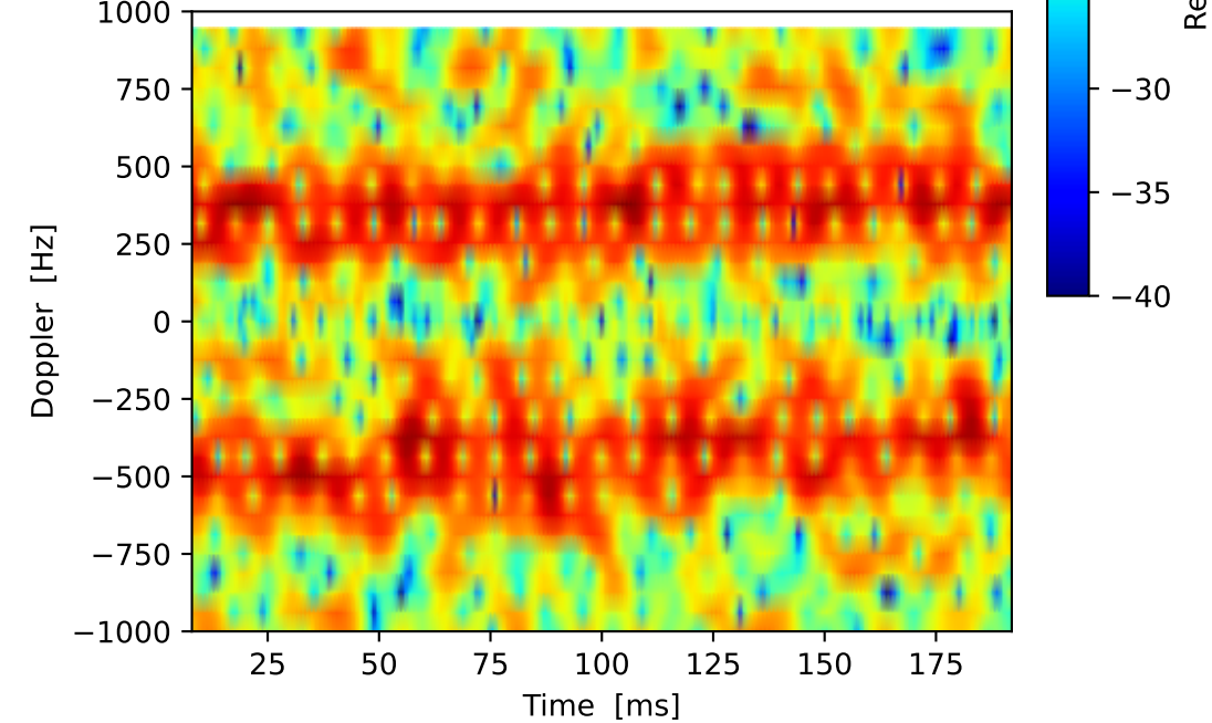
(i) 5G frame rate 2 kHz — micro-Doppler aliases
