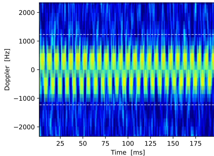
(e) Passive chain, ideal reference
