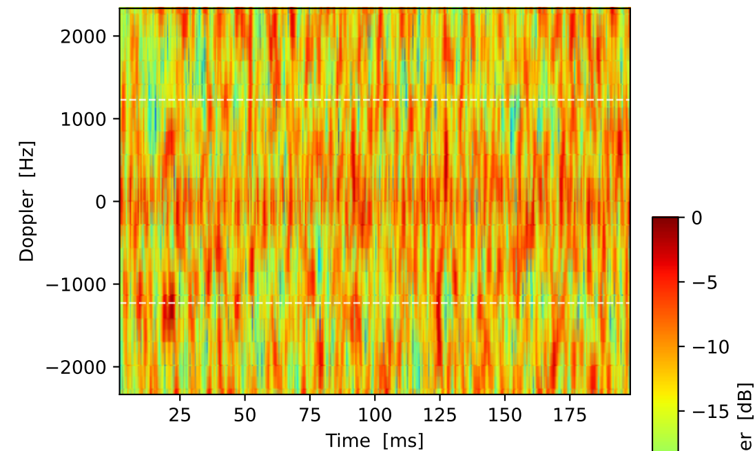
(f) Passive chain, reference SNR 10 dB
