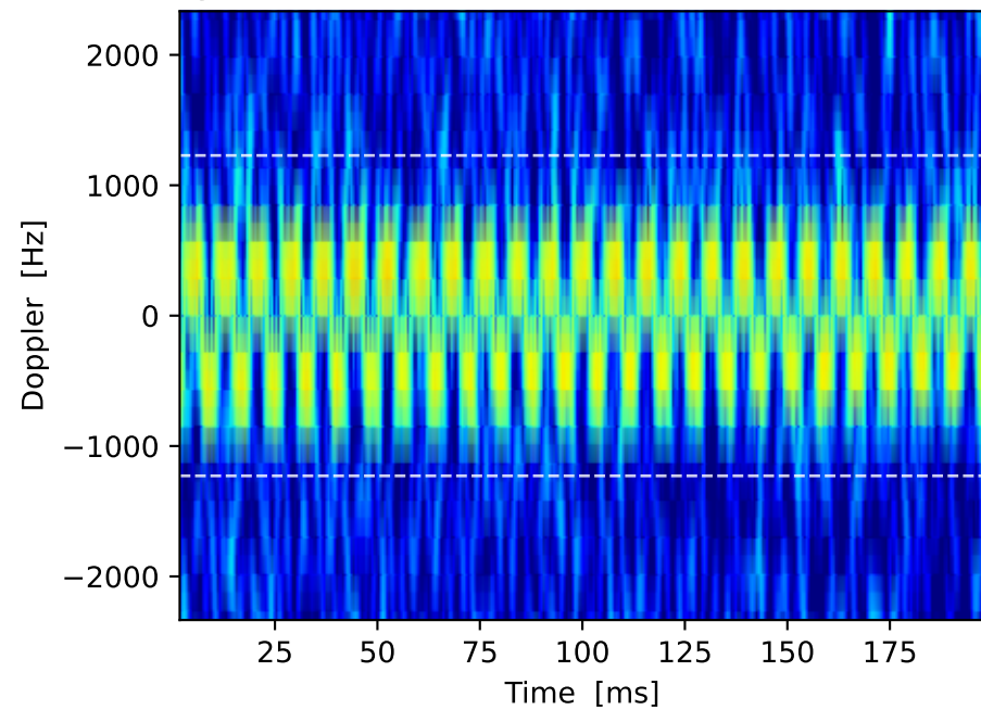
(g) Passive chain, multipath reference -20 dB
