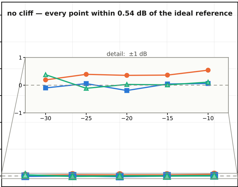
(b) reference-channel multipath — same vertical scale
