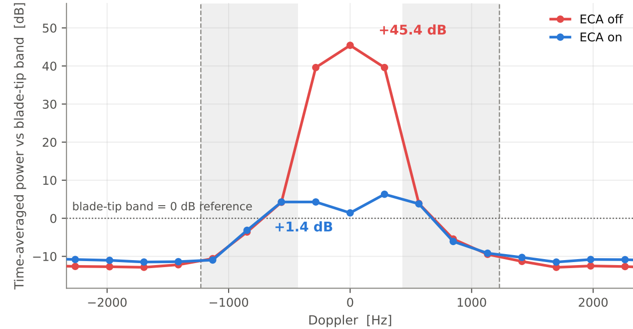
(c) What ECA removes — direct path present, WiFi chain
