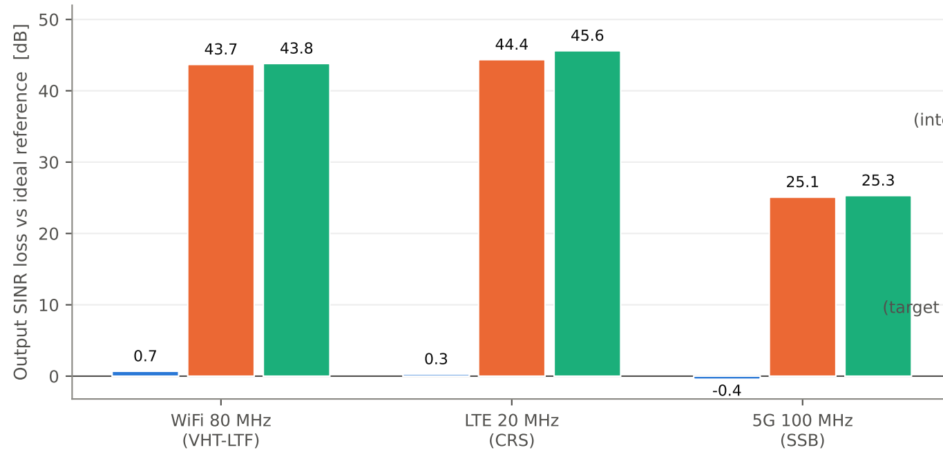
(b) The same decomposition at reference SNR 10 dB
