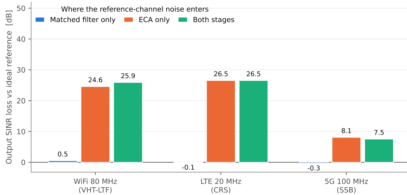
(a) Contaminating one stage at a time — reference SNR 20 dB
