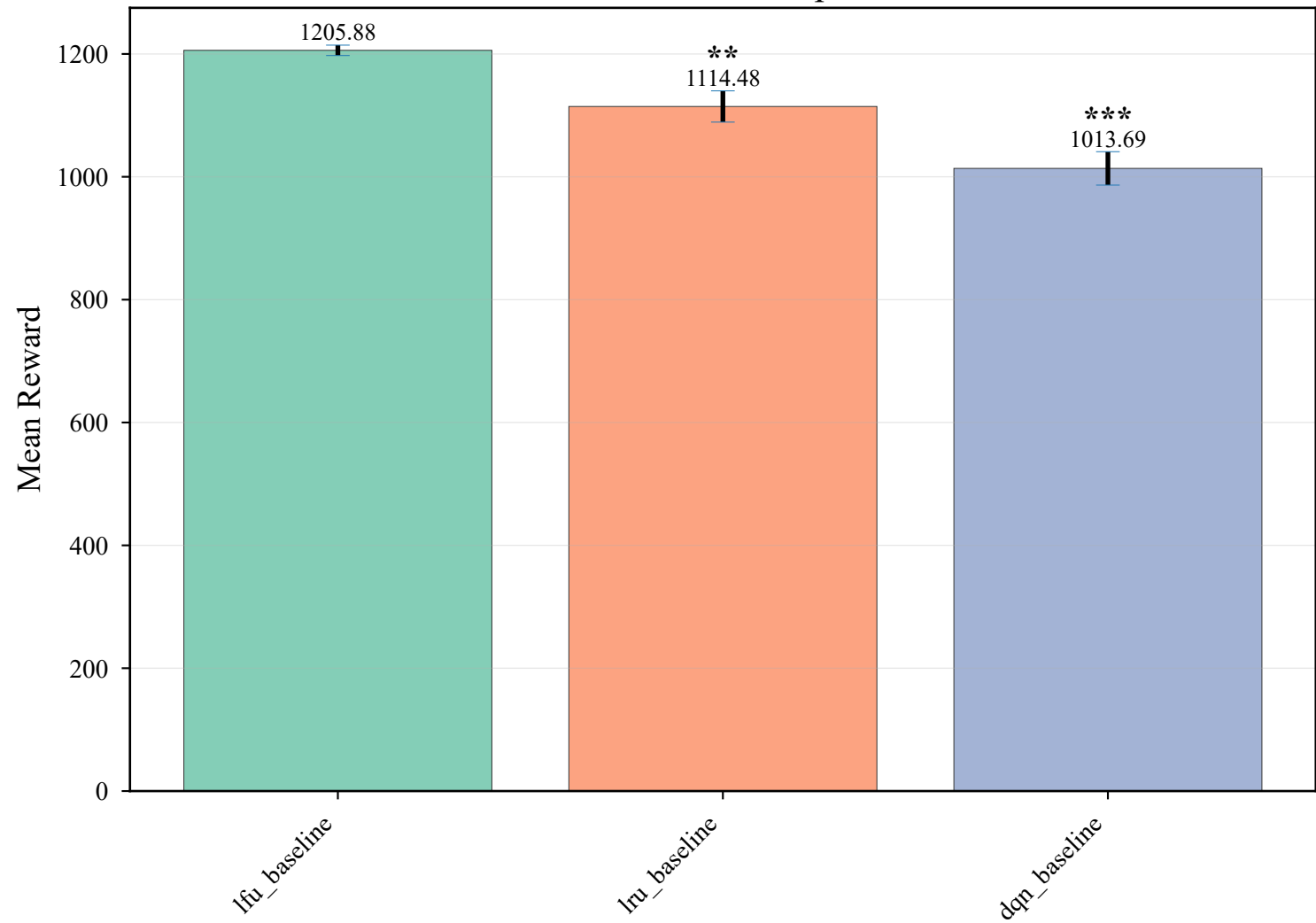
Mean Reward Comparison
