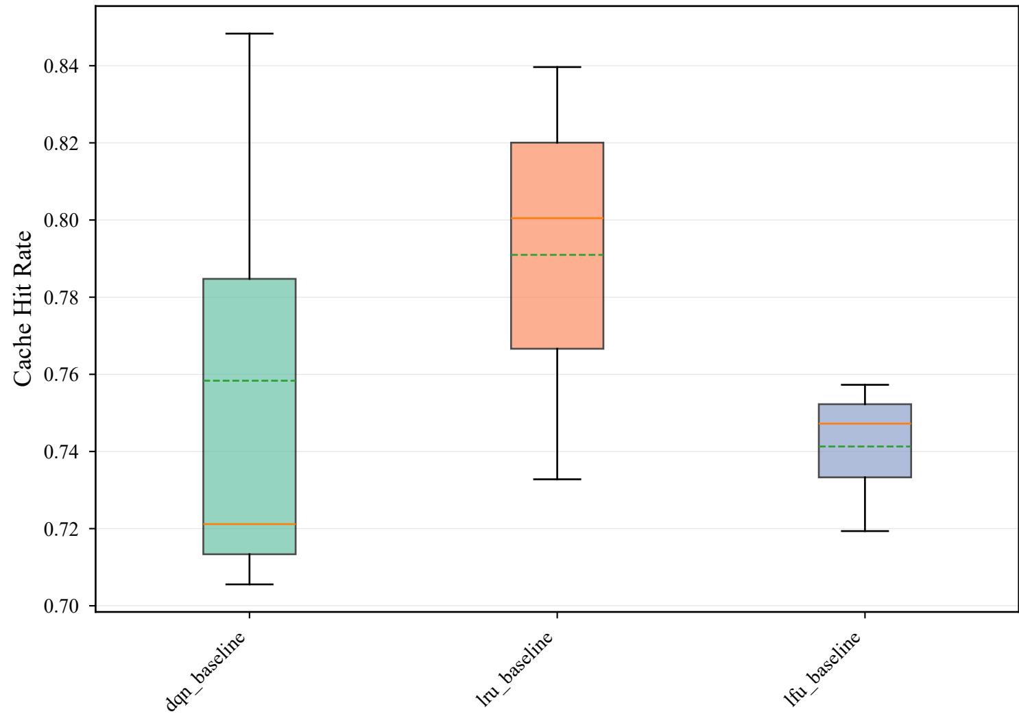
Cache Hit Rate Distribution
