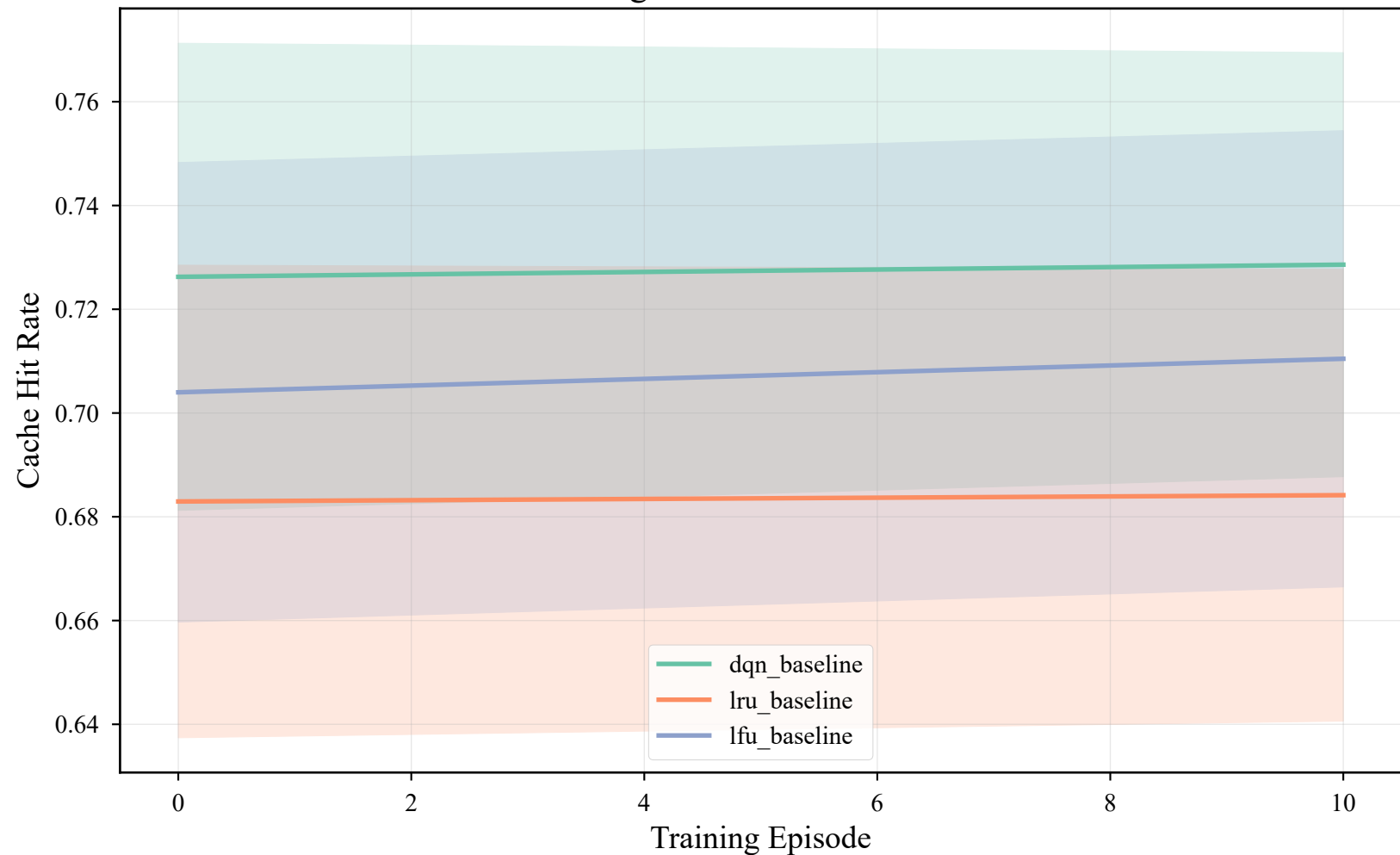
Learning Curves: Cache Hit Rate
