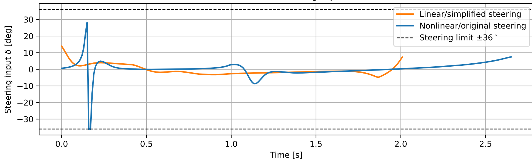
Controller Steering Input
