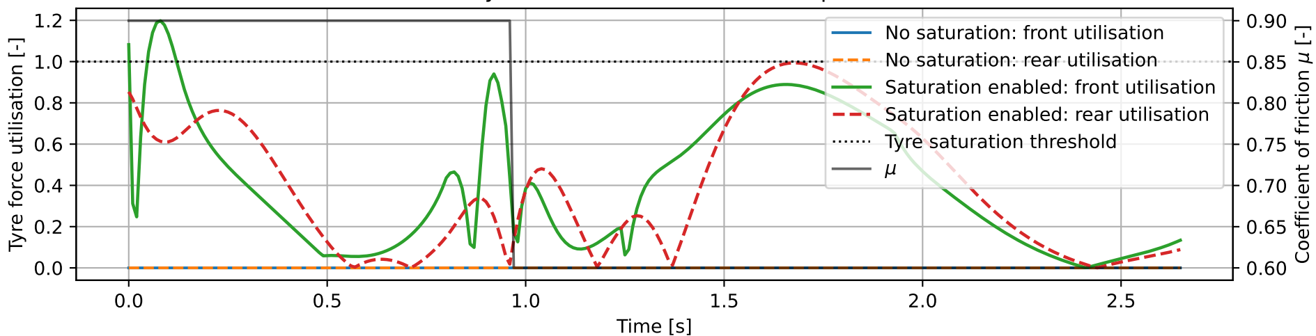
Tyre Utilisation and Friction Step
