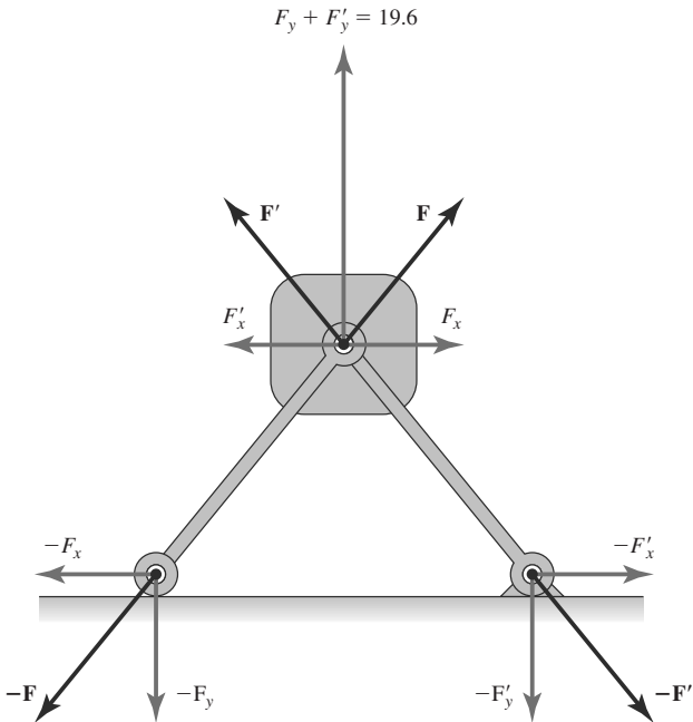
FIGURE 1-18 The force on the weight and the forces on the roller and pivot,
