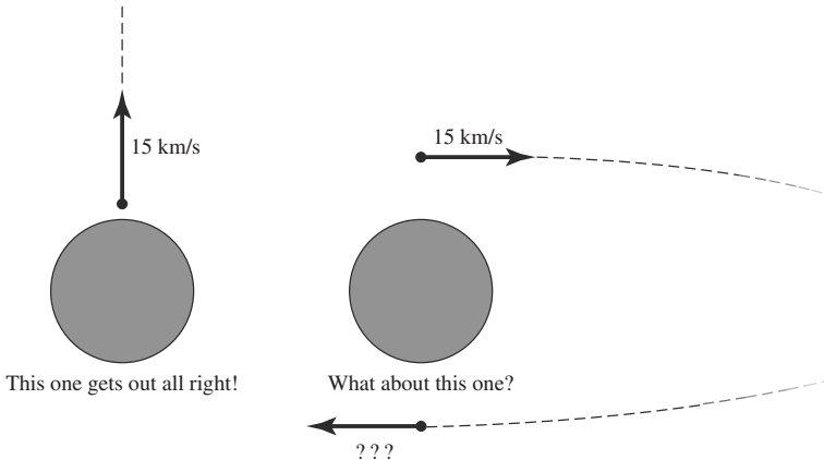
FIGURE 2-12 Does having the escape velocity guarantee escape?
