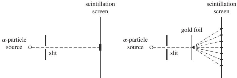
FIGURE 3-8 Rutherford's experiment deflecting alpha particles, which led to
