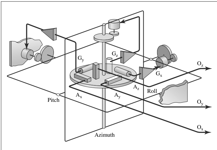
FIGURE 4-21 A complete navigational system, with three gyroscopes and three
