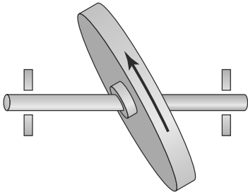
FIGURE 4-29 Spinning the disk around its main axis with angular velocity \Omega ,
