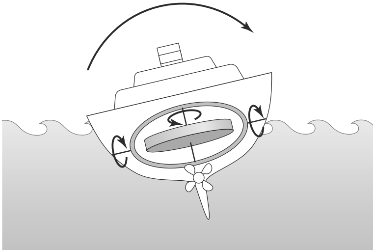
FIGURE 4-4 A ship-stabilizing gyroscope: pitching the gyroscope forward
