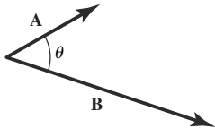
FIGURE 1-10 The vector dot product |\mathbf{A}||\mathbf{B}|\cos\theta is the same in all coordinate
