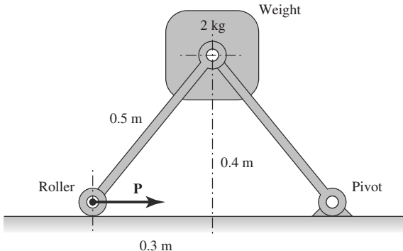
FIGURE 1-16 What force, P , is required to hold up the weight?
