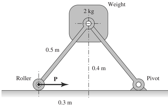
FIGURE 2-4 The simple machine of Chapter 1.
