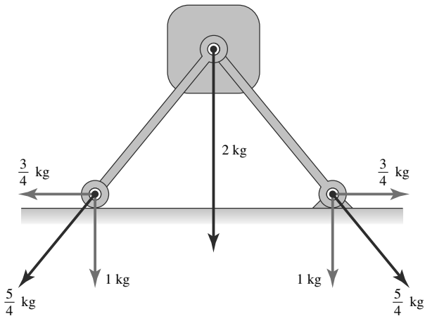
FIGURE 2-5 Distribution of force from the weight, through the rods, to the
