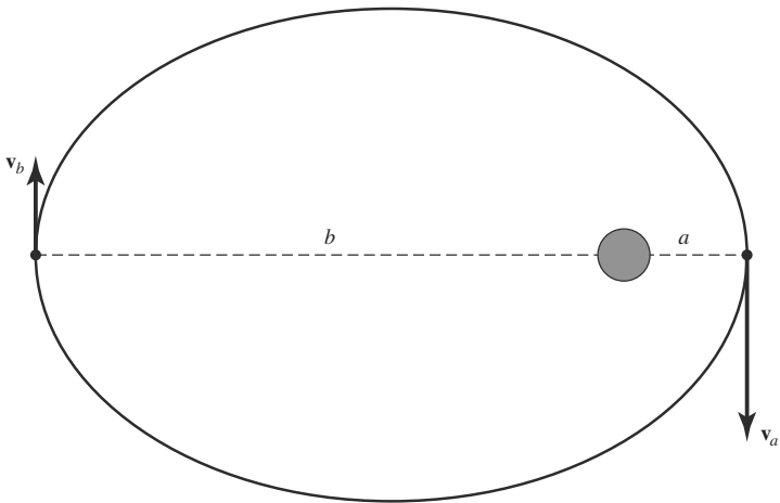
FIGURE 3-2 Velocity and distance at perihelion and aphelion of a satellite in an
