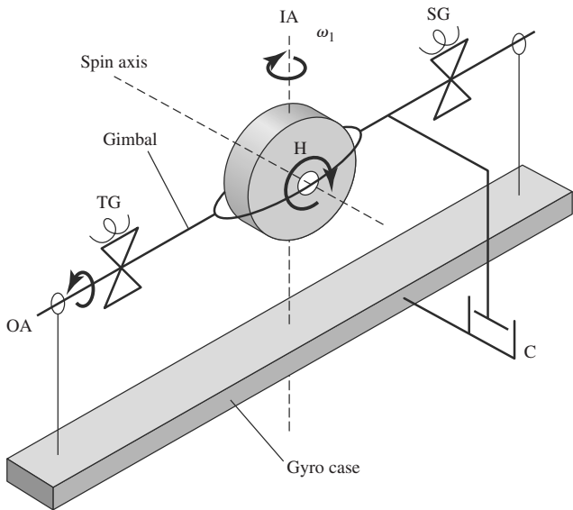
FIGURE 4-10 Simplified schematic of a one-degree-of-freedom gyroscope.
