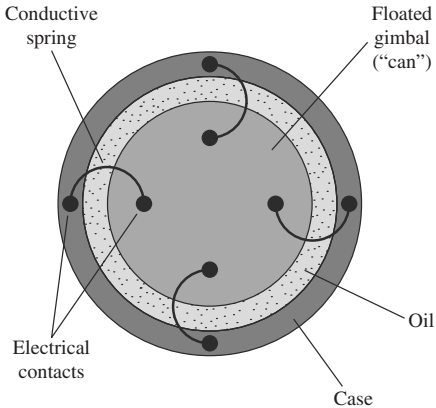
FIGURE 4-14 Electrical connections from the case to the floated gimbal in a
