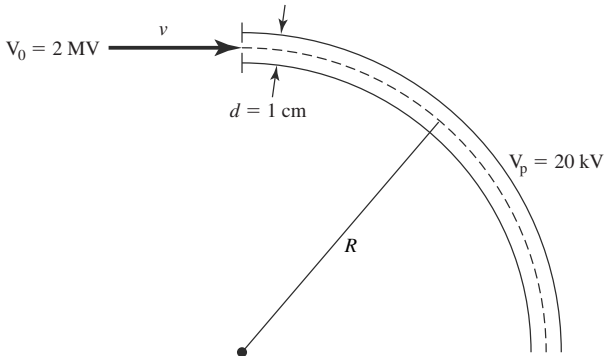
FIGURE 3-12 Electrostatic proton beam deflector.
