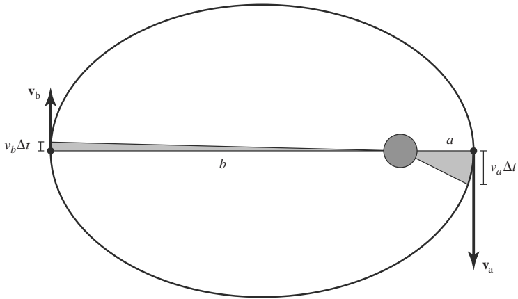
FIGURE 3-4 Using Kepler's law of equal areas to find the velocity of a satellite at
