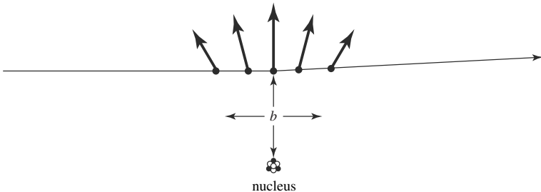
FIGURE 3 - 6 The electric force of the nucleus effectively acts on the proton for a
