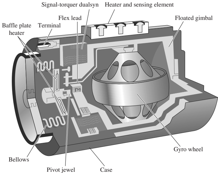
FIGURE 4-13 Cutaway view of an actual one-degree-of-freedom integrating
