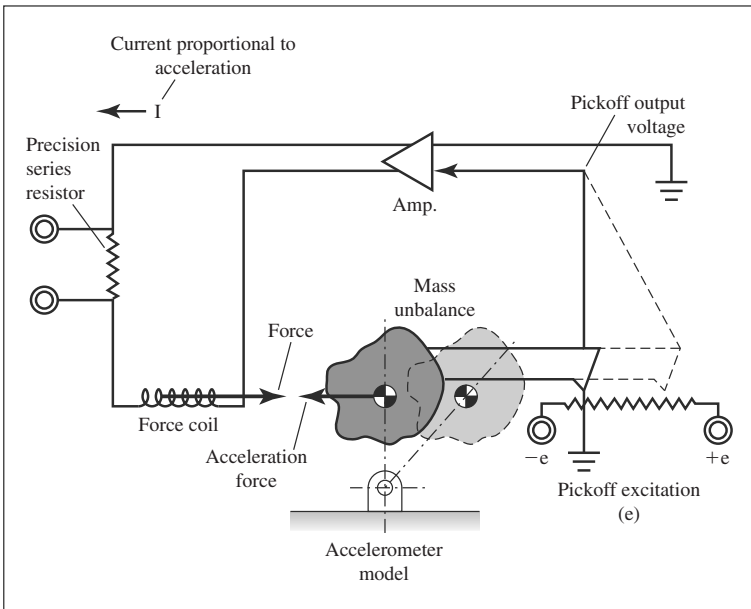
FIGURE 4-17 Schematic of an unbalanced mass accelerometer with force
